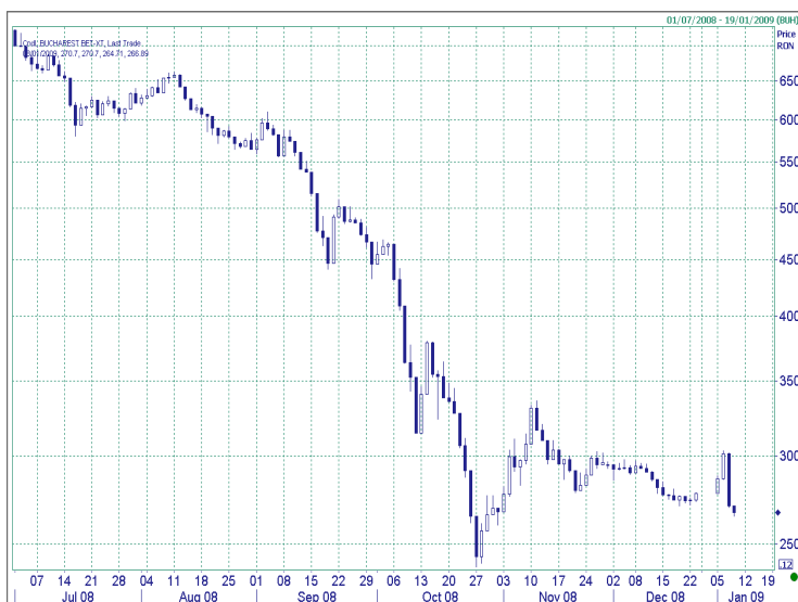
Indicele BET-XT
