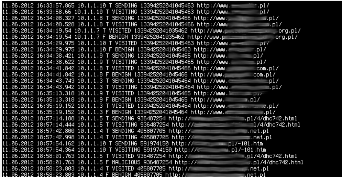
Figure 33: Capture-HPC NG in operation (screenshot)
