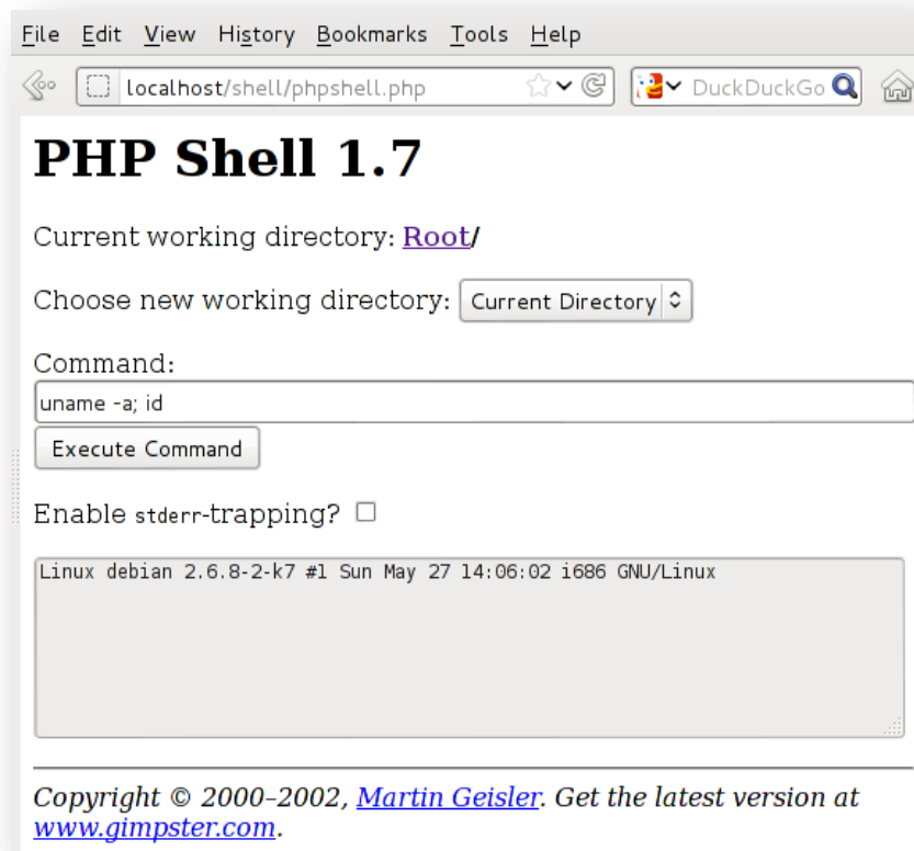
Figure 20: Google Hack Honeypot in operation (screenshot)
